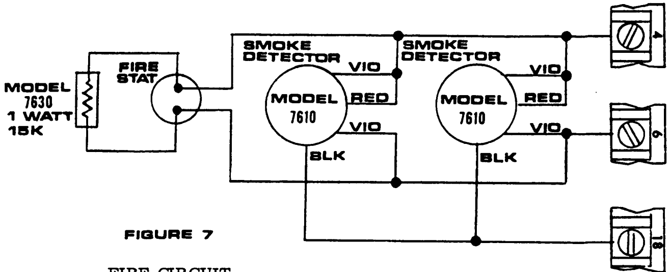
FIRE CIRCUIT
